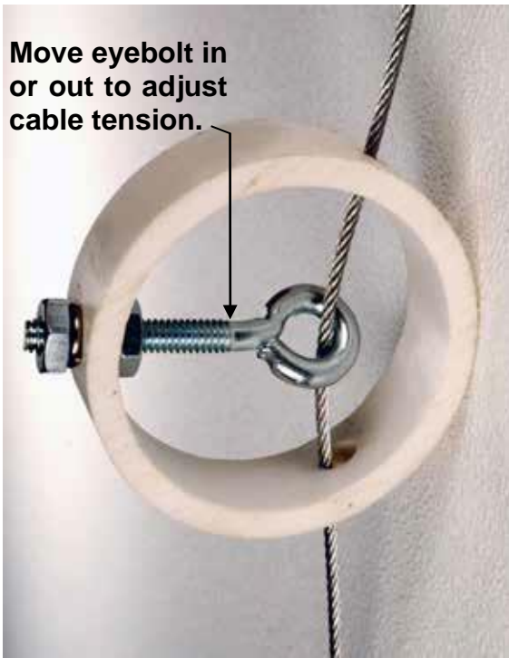
(Cable Adjuster Assembly)
