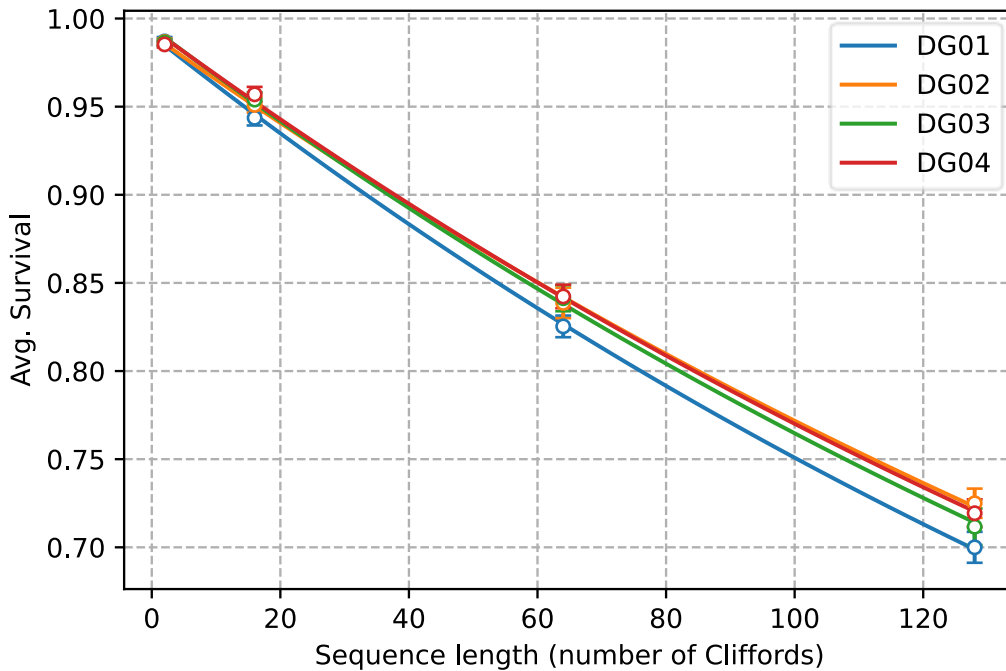
Figure 4: Two-qubit RB results from H2-1 taken on 2023/03/20.
