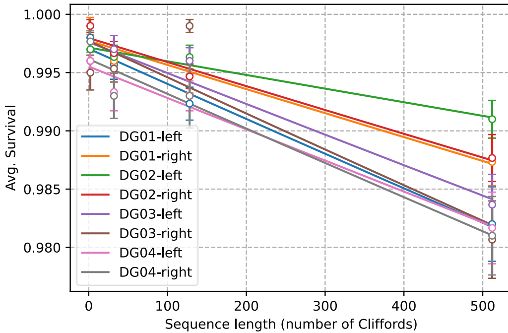
Figure 3: Single-qubit RB data from H2-1 taken on 2022/02/07.
