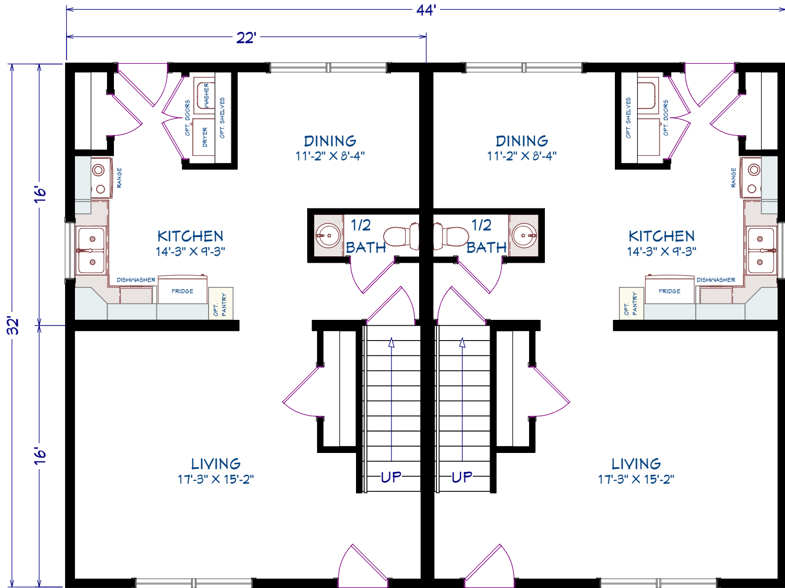
MAIN FLOOR 2 LEVEL DUPLEX, 2 BEDROOM UNITS 704 SQ FT
