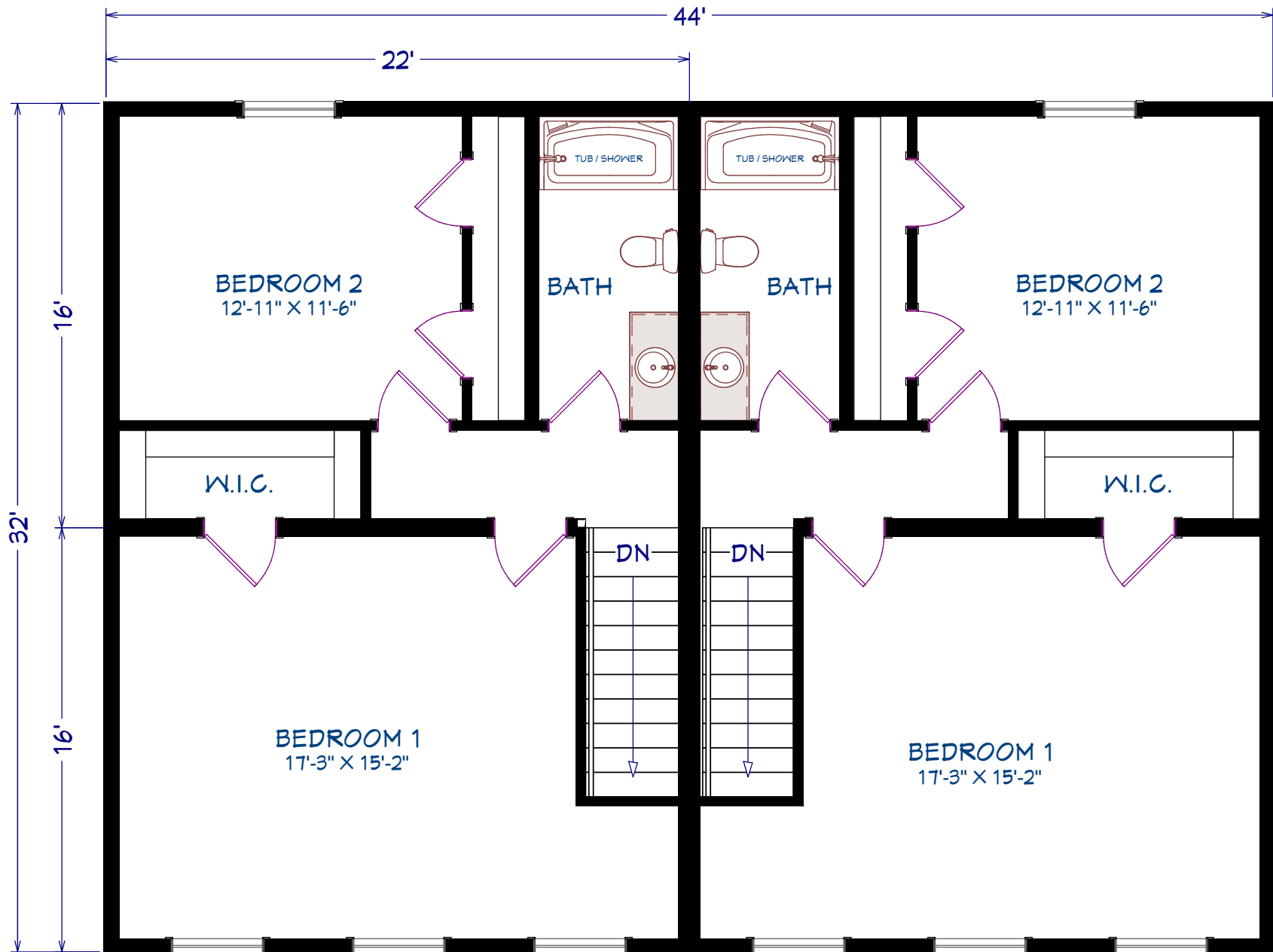
SECOND FLOOR 704 SQ FT
