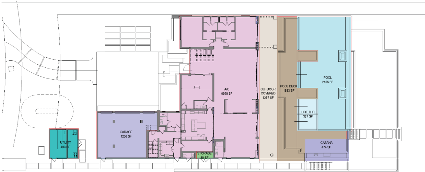
2 AREA PLAN LEVEL 1 1/16" = 1'-0"
