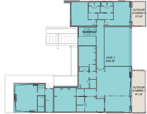
3 AREA PLAN LEVEL 2 1/16" = 1'-0"
