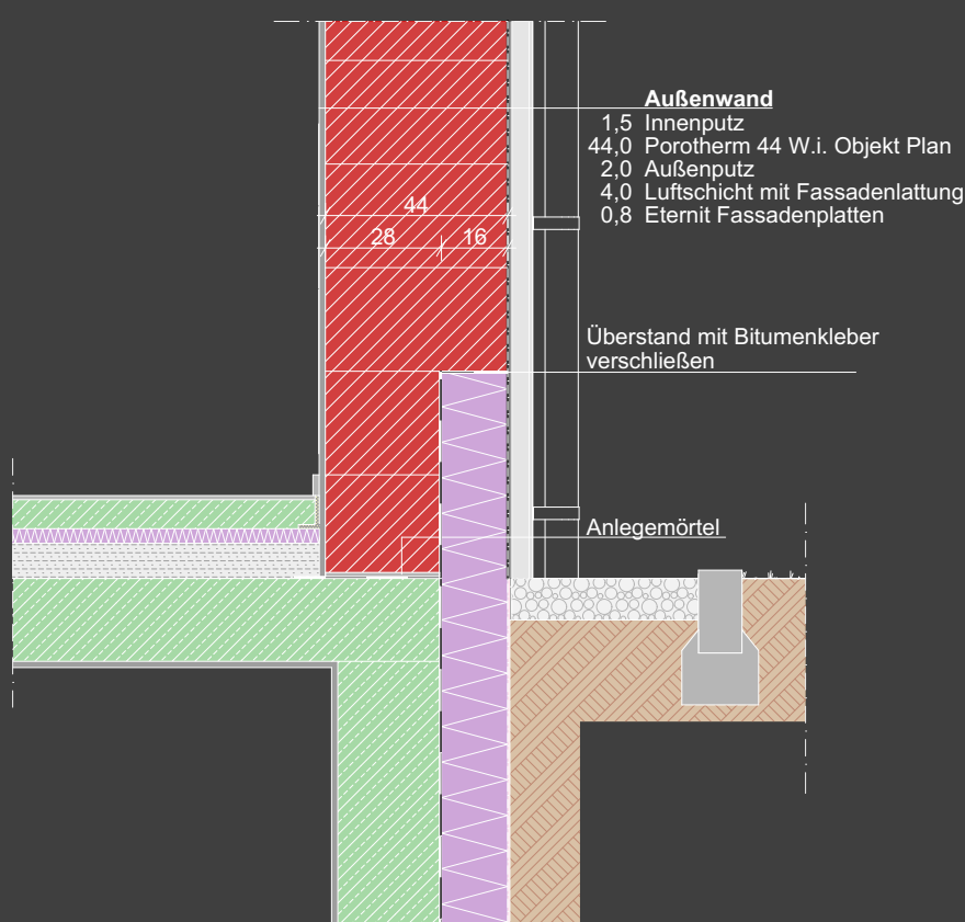
1:20 Sockeldetail
