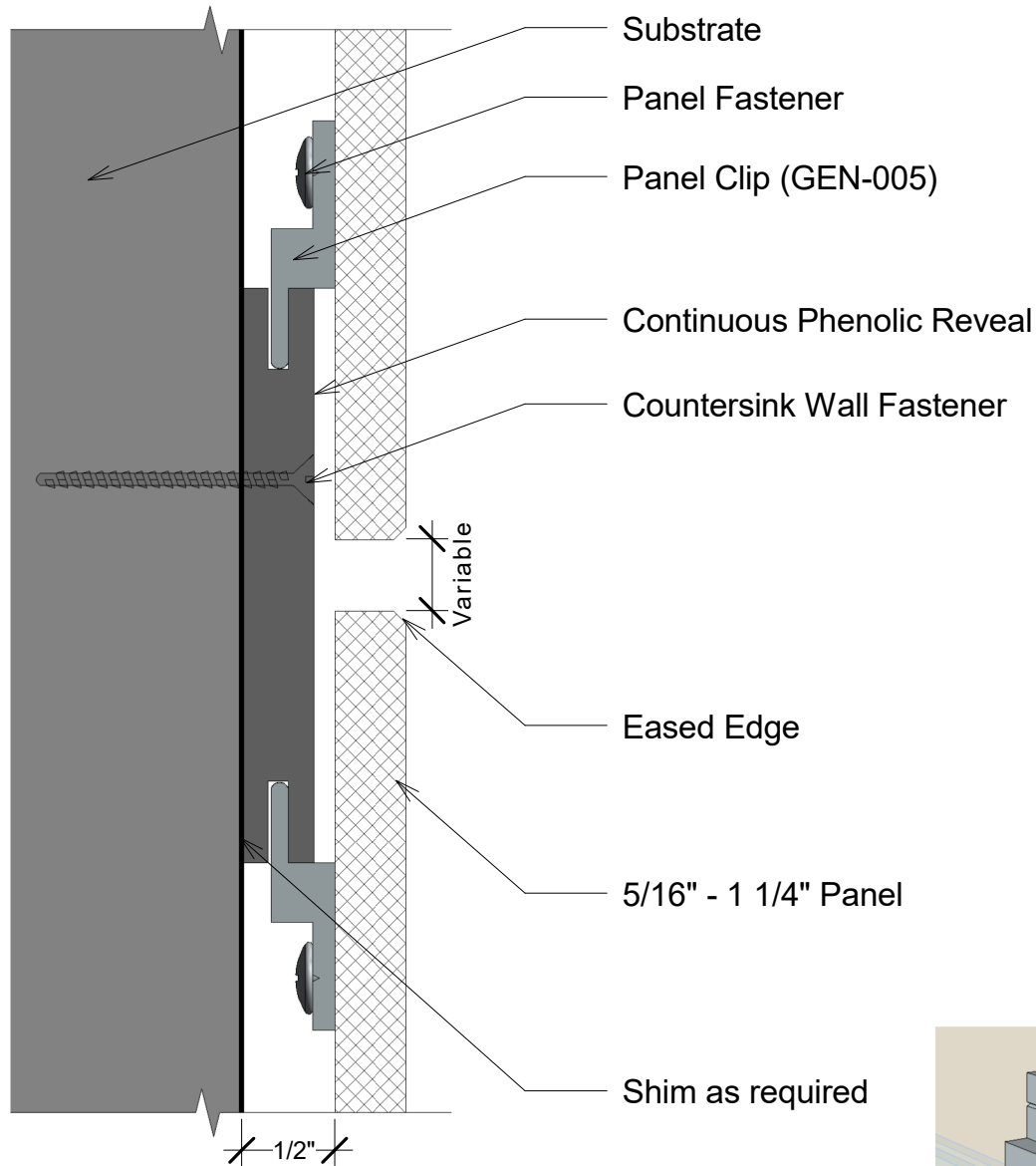
1 Section J 12" = 1'-0"
