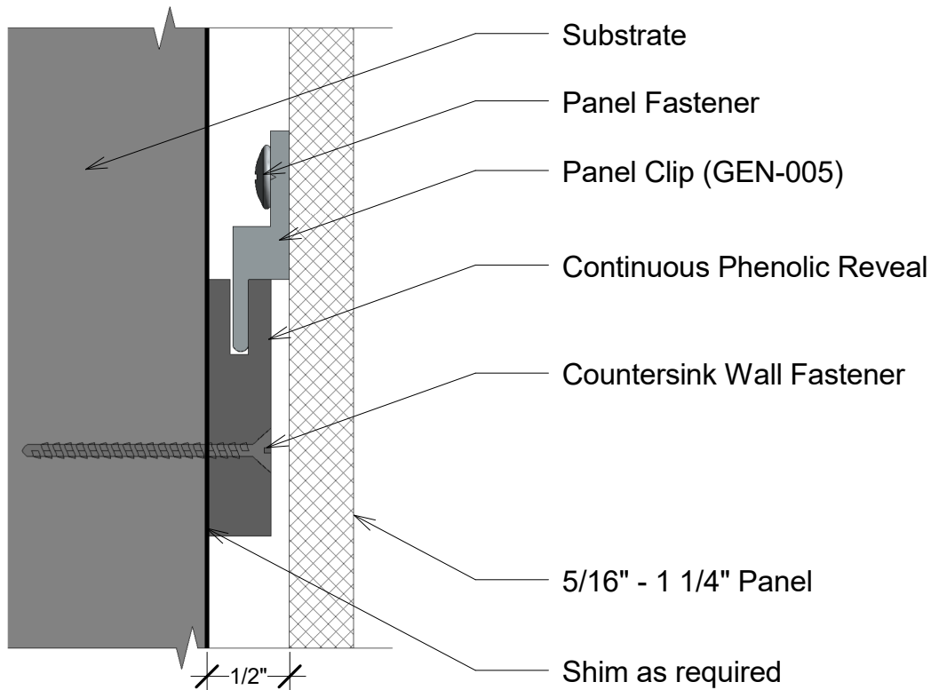
1 Section L 12" = 1'-0"
