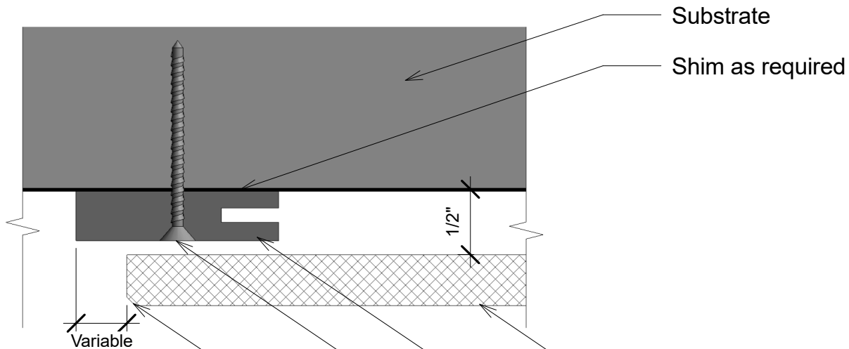
1 Plan View - A 12" = 1'-0"
