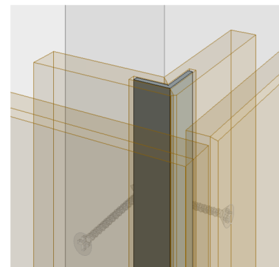
② Alumium Spline Joint (G)
