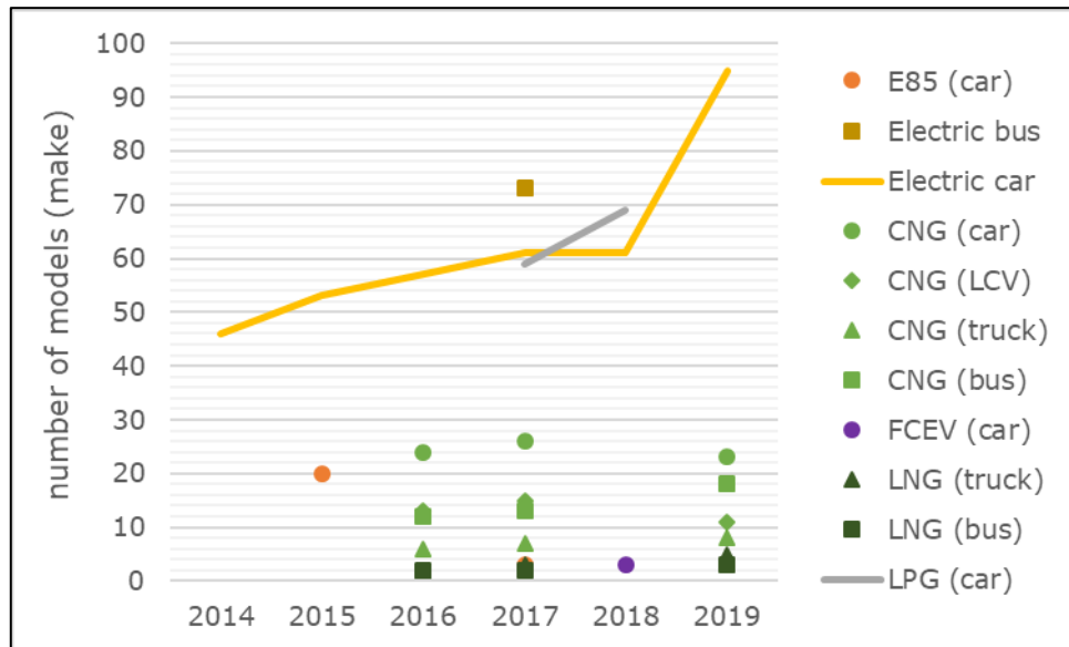
Figure 6-1. Alternative fuels vehicle model availability
