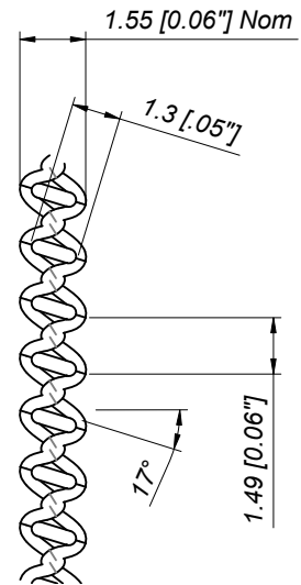
Detail B Scale:5:1
