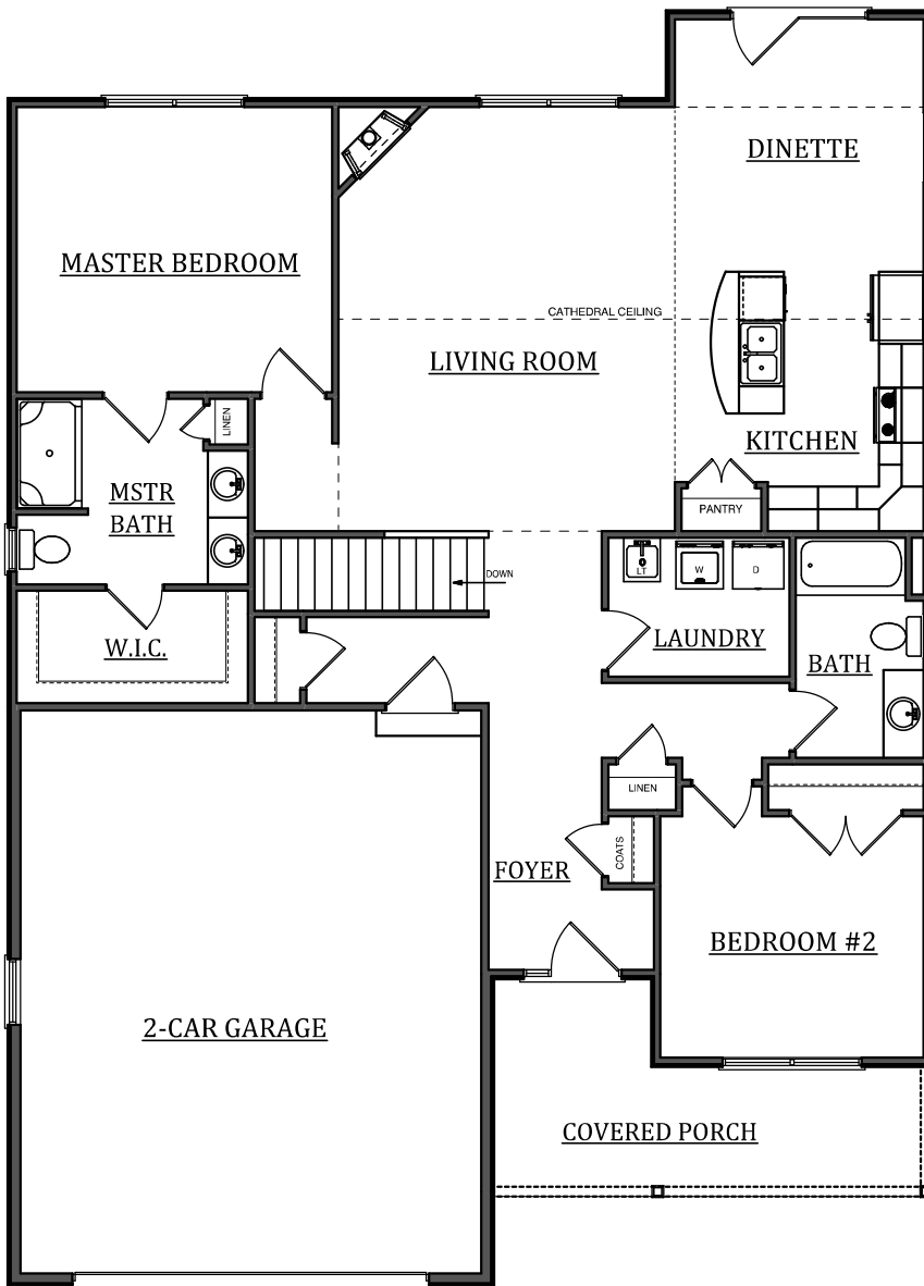
MAIN FLOOR PLAN 1,517 Sq. Ft.
