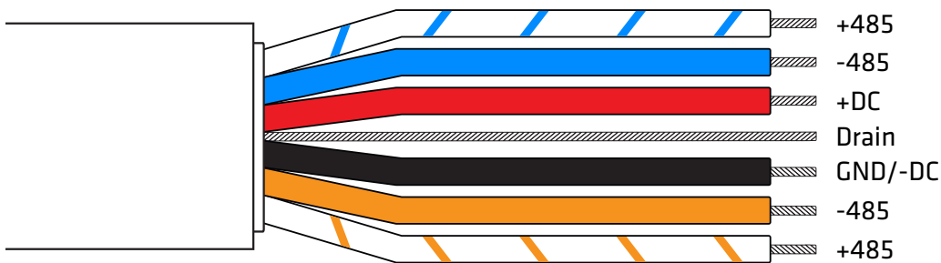
Matrix Rail homerun cable
