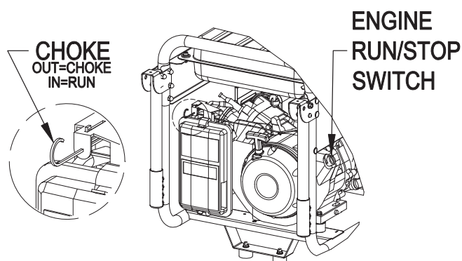
Figure 12 - Choke Position
