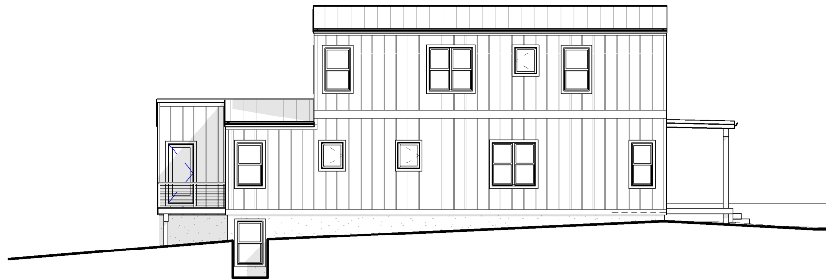
SIDE ELEVATION
