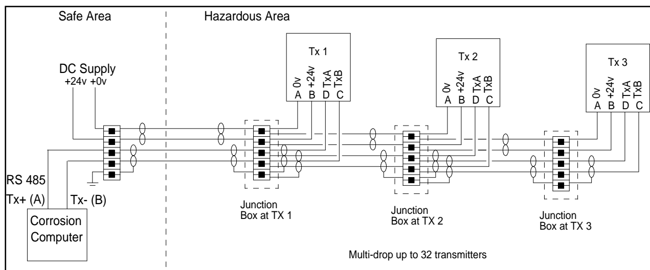
Figure 7 Multi-drop wiring
