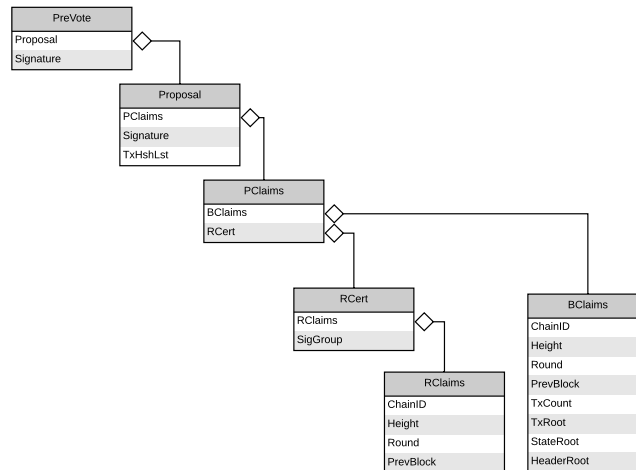
Figure 9: PreVote Object
