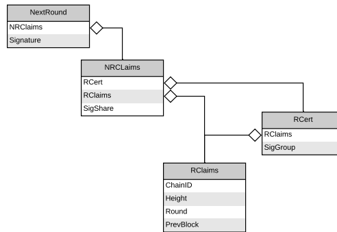
Figure 13: NextRound Object
