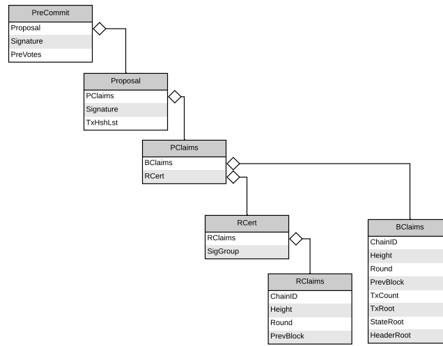
Figure 11: PreCommit Object
