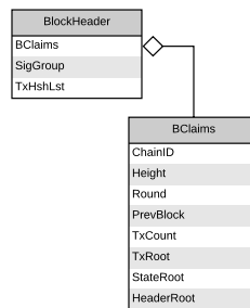
Figure 15: BlockHeader Object
