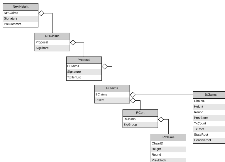
Figure 14: NextHeight Object
