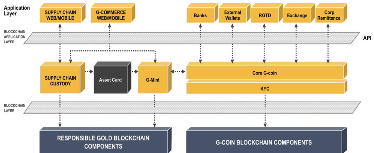
Figure 14: RG Supply Chain and Application Layers in RG Ecosystem
