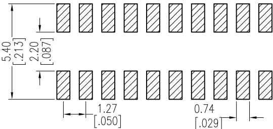
Recommended P.C.B Layout(Top Side) (PCB BOARD TOLERANCE±0.05)
