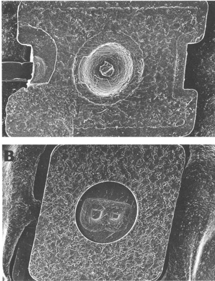
Figure 5 Scanning electron micrograph showing the design of the bases of the plastic brackets (A) Dentaurum Edgewise and (B) Spirit.
