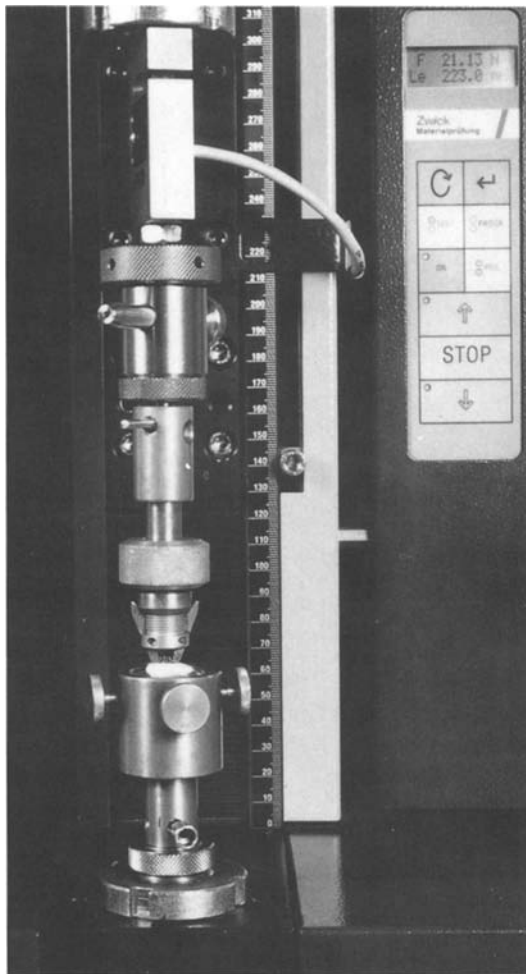
Figure 1 Experimental set up in the universal testing machine.
