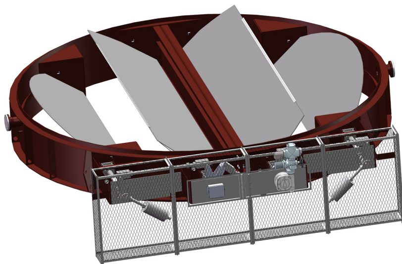
Custom stack damper with guards around linkages.
