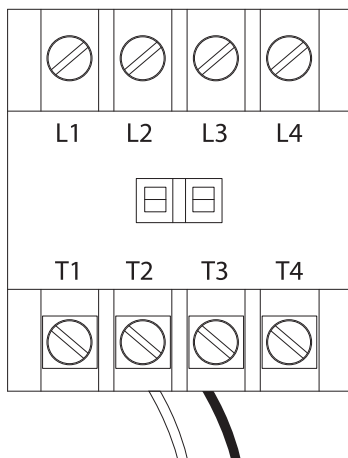
Detail 1. DT-XP40A Contactor
