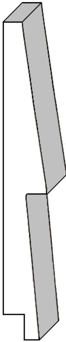
HDM 55 LAP 3/4" x 5-1/2"
