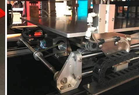
adjustable gathering table
