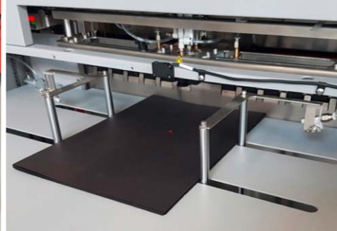
feeder for cardboards
