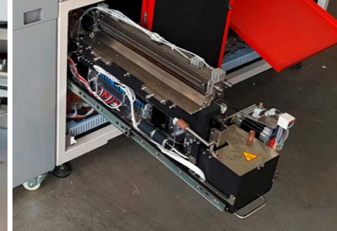
removable glue roller with glue tank
