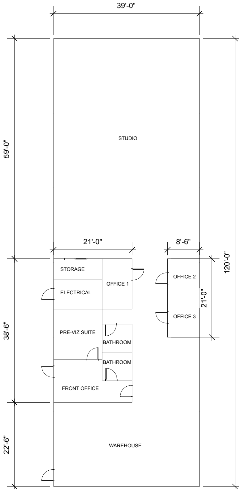
1 Plan View Scale: 1/16" = 1'-0"
