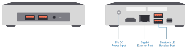
Figure: Mezzanine 200 Series: Perception Appliance Interfaces
