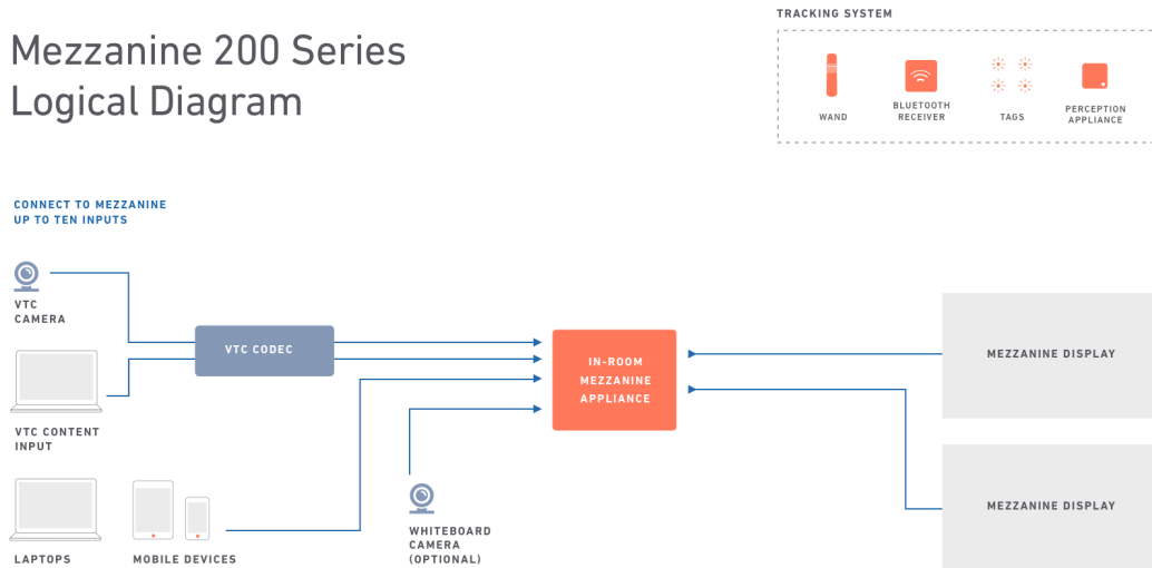
Figure: Mezzanine 200 Series: Logical Diagram
