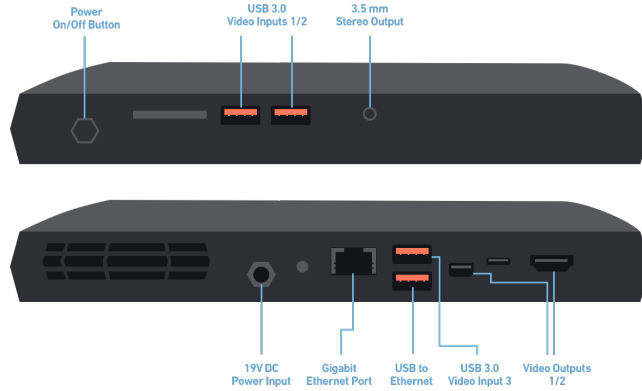
Figure: Mezzanine 200 Series: Mezzanine Appliance Interfaces
