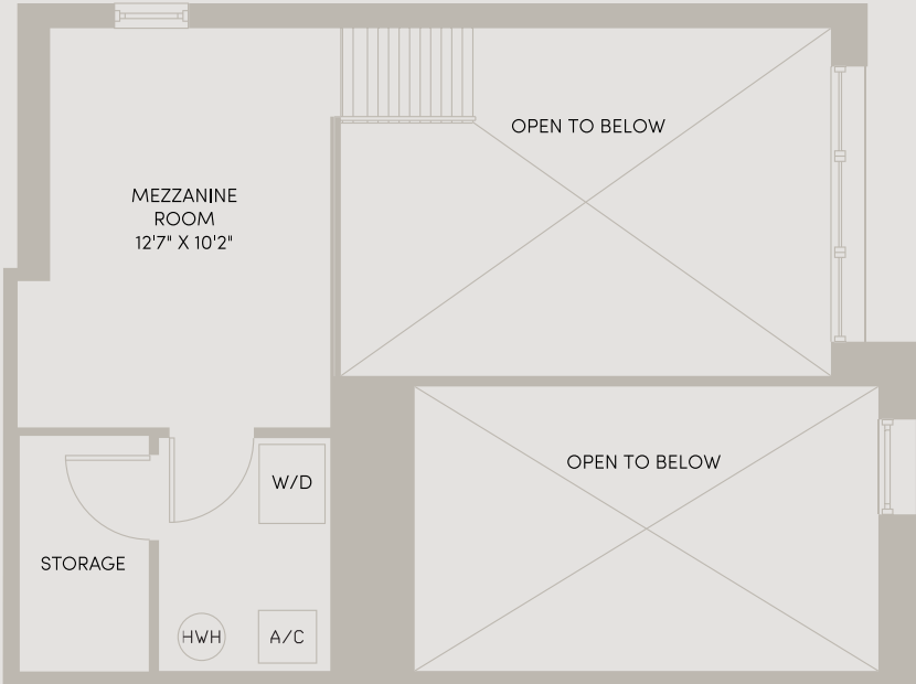
MEZZANINE LEVEL
