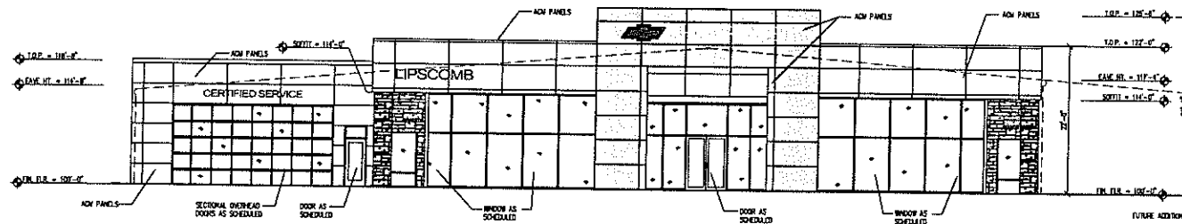
1 FRONT (WEST) ELEVATION
