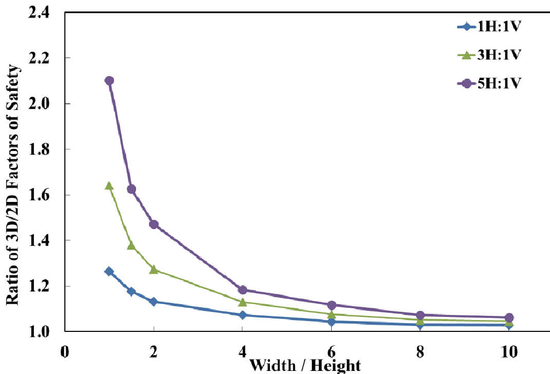
Figure 1. Relationship between 3D and 2D FS ( R_{3D/2D} ) as a Function of Slide Configurations (from Akhtar and Stark 2017)
