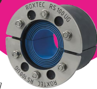
RS-seal (UG)
