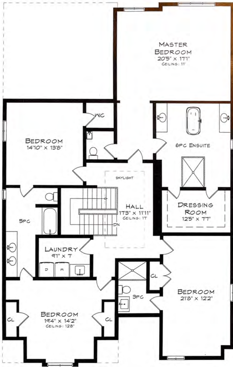
UPPER LEVEL 2,235 SQUARE FEET
